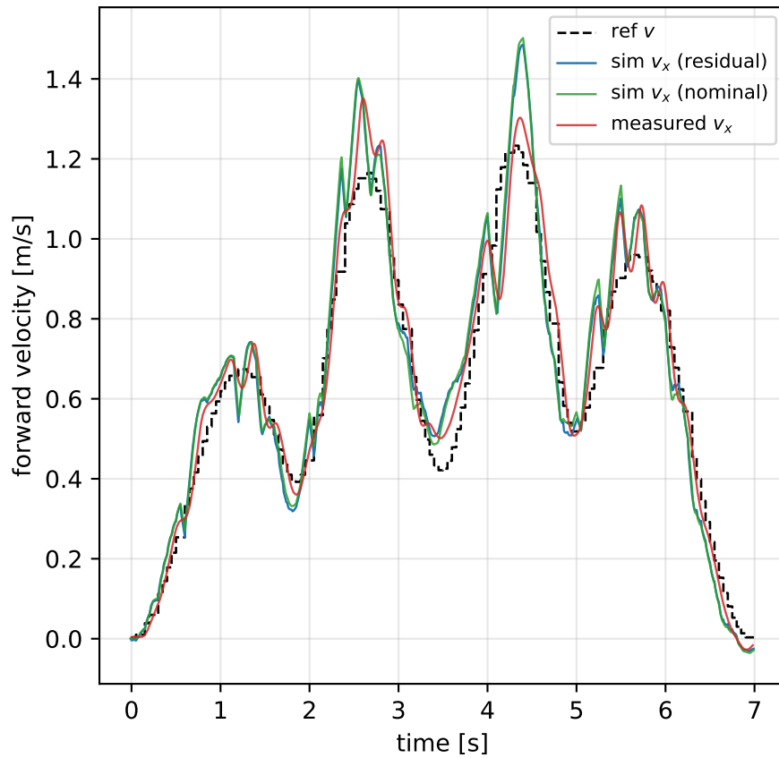
Closed-loop simulation with residual model vs measured log
